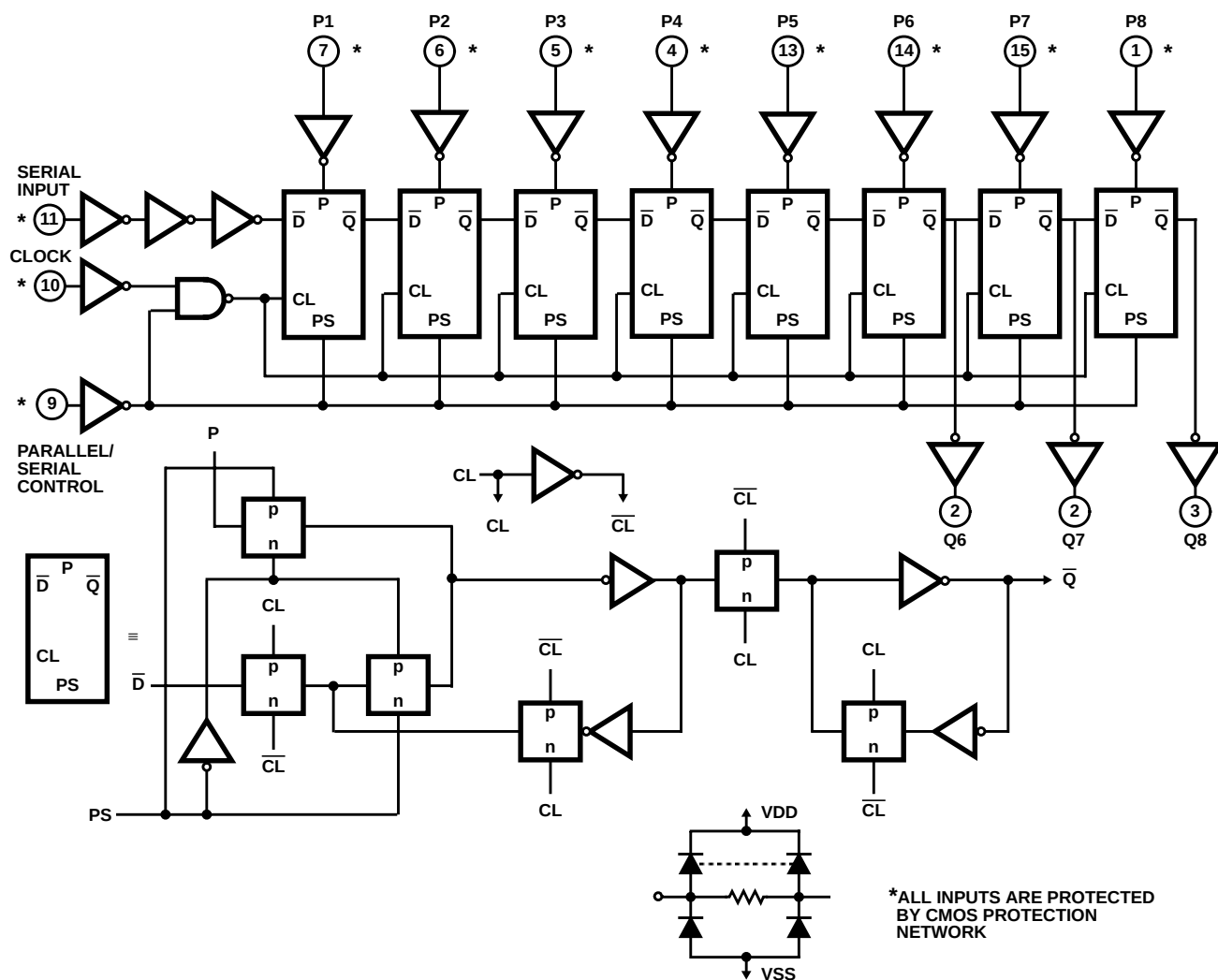
FIGURE 2. CD4021BMS LOGIC DIAGRAM
