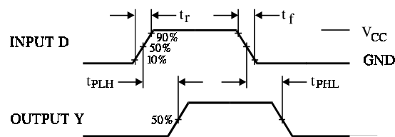
Figure 1. Switching Waveforms
